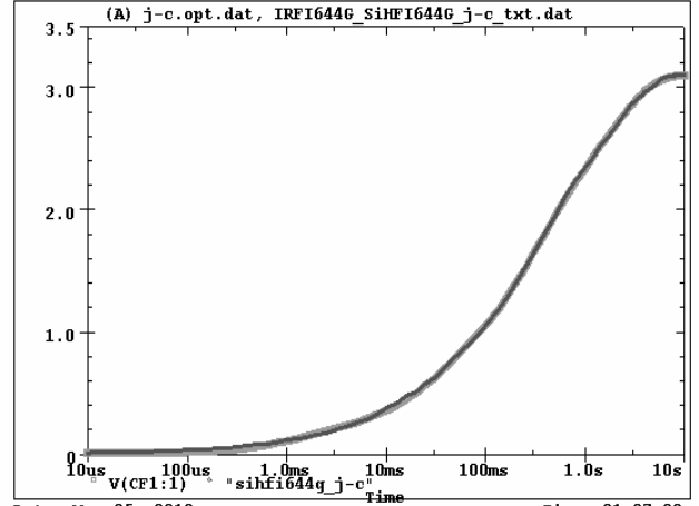
IRFI644G_SiHFI644G Filter j-c Temperature: 27.0
