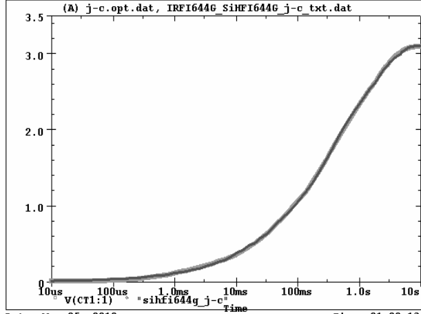
IRFI644G_SiHFI644G Tank j-c Temperature: 27.0
